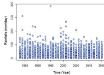
Figure 3 The plot of daily rainfalls in Makassar Municipality, 1985-2015
