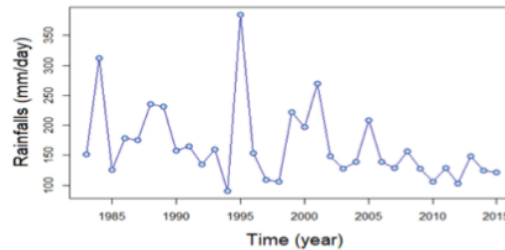
Figure 3 Extreme rainfall series data in Makassar Municipality using AM Approaches.
