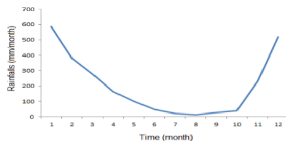
Figure 1 Plot of Monthly mean rainfalls in Makassar Municipality.
